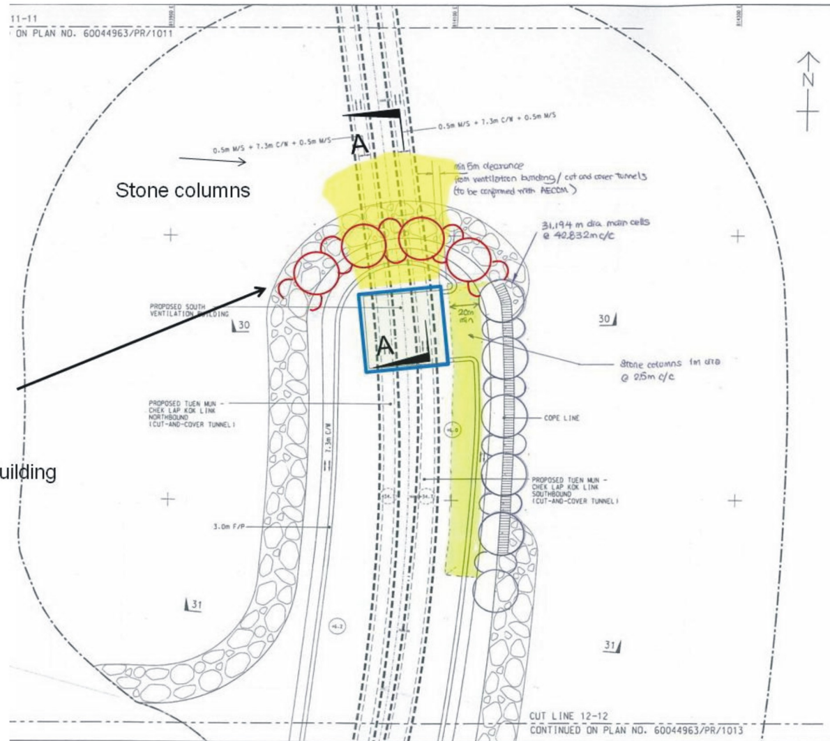
Figure 22 - Interface to TM-CLKL Tunnel Sections (Sheet 1 of 2)
